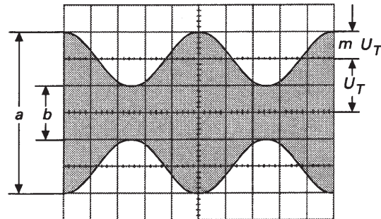
Figure 2: Amplitude modulated oscillator:
