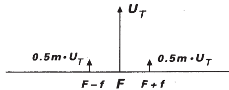
Figure 1: Amplitude and frequency spectrum for AM display ( m = 50\% )
